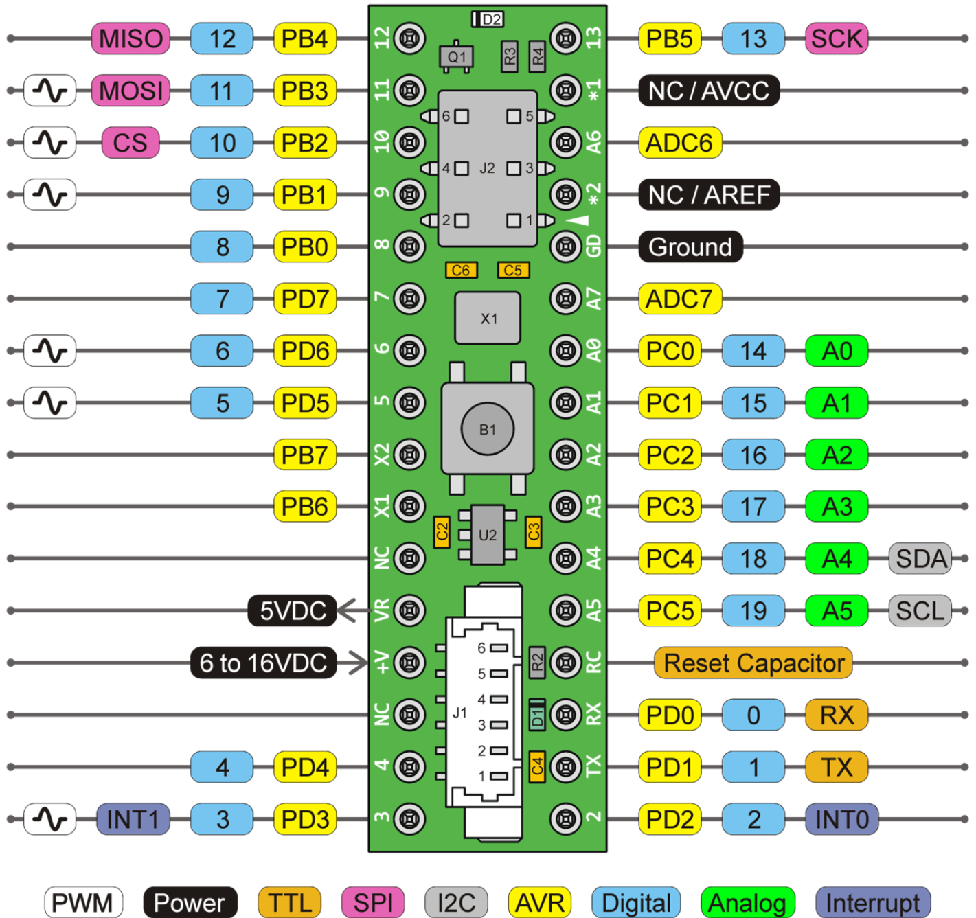
Figure 1 P1 Header Pins
