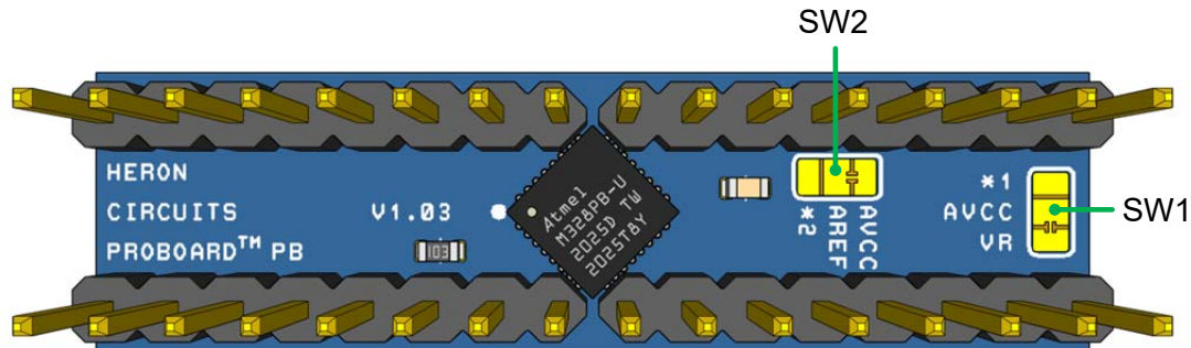
Figure 5 Configuration Switches
