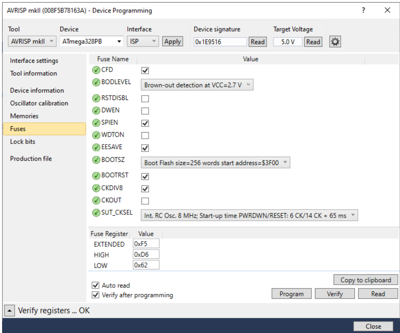
Figure 9 Low Power Fuse Settings
